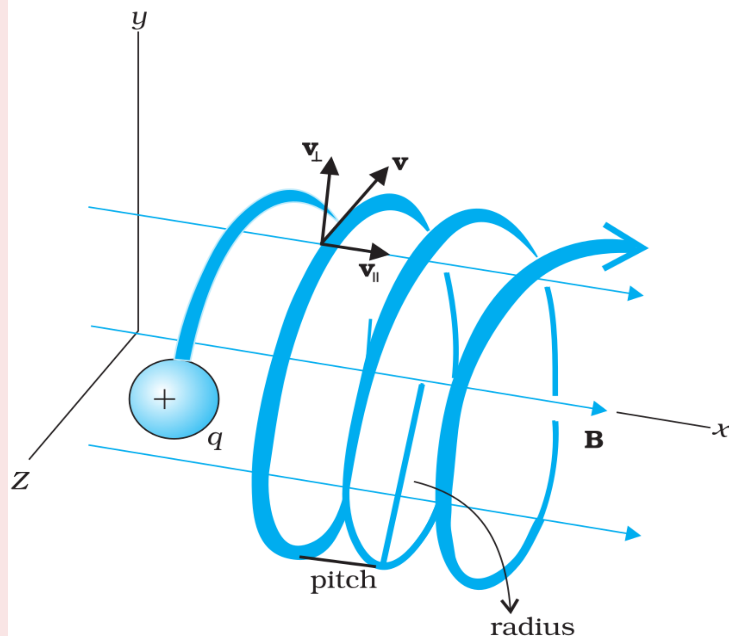
FIGURE 4.6 Helical motion
