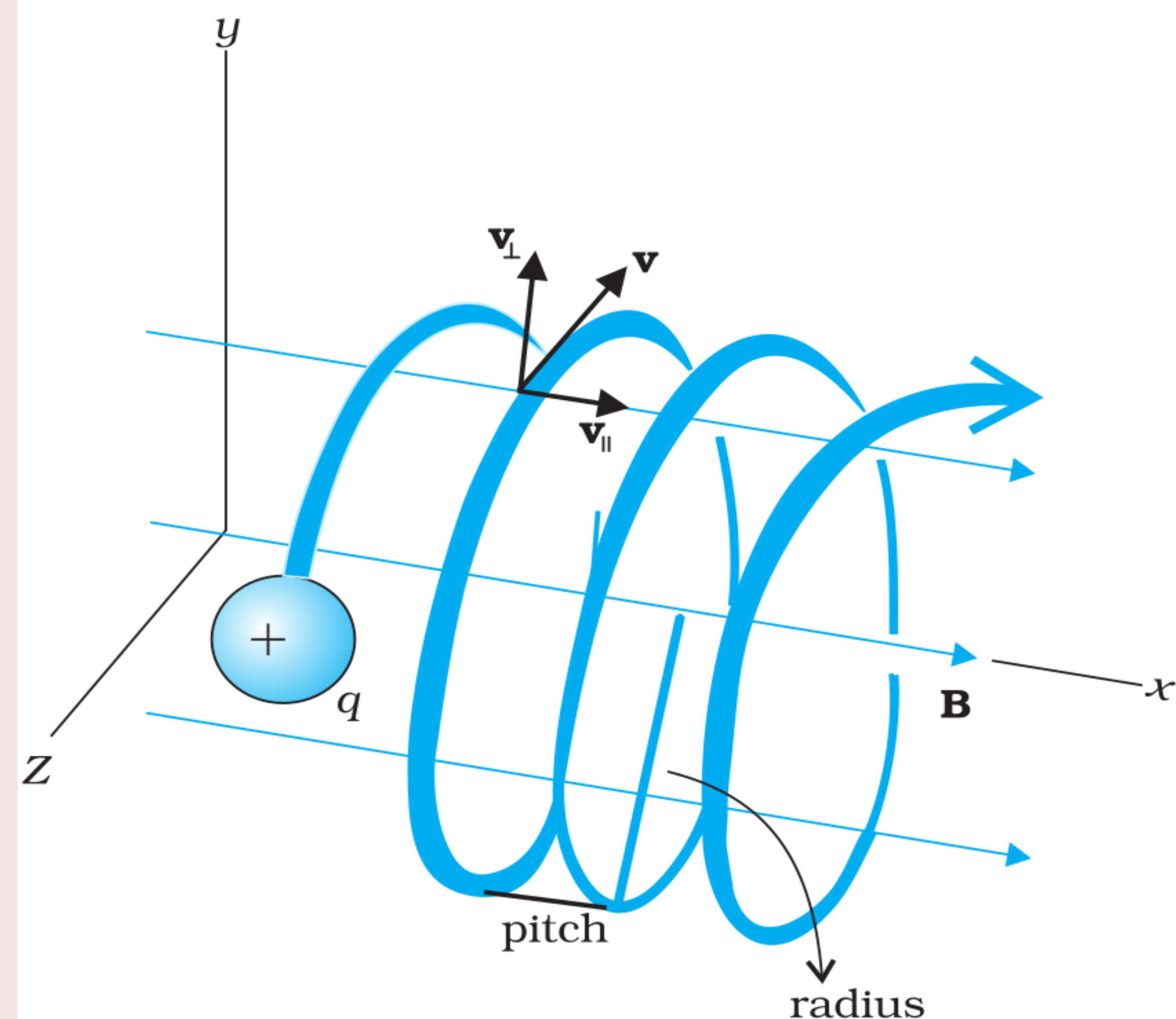
FIGURE 4.6 Helical motion
